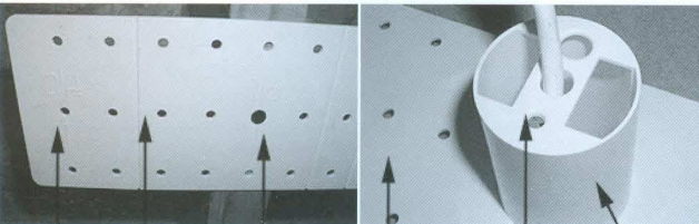
24" Center Mark Break Point 16" Center Mark Bridge Wire Inlet Holes Wire Cavity
